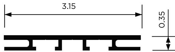
80mm SEG BENDABLE (LIGHTBOX COMPATIBLE)
