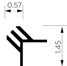
CORNER CLADDING
