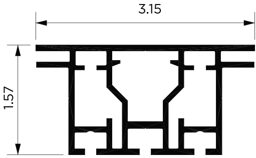
80mm SEG EXTRUSION
