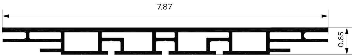
200mm SEG EXTRUSION (LIGHTBOX COMPATIBLE)
