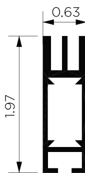
CUBE EXTRUSION
