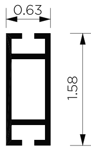
RAIL EXTRUSION
